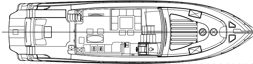
MAIN DECK
